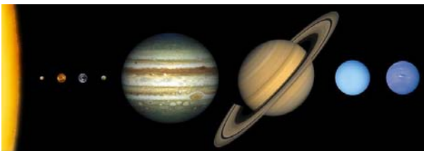
Solar System
