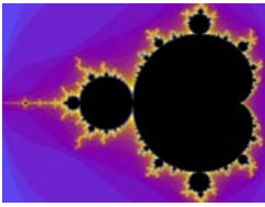
Mandelbrot Set
